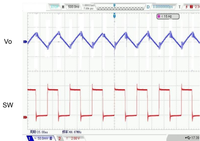
5. Switching Waveform
